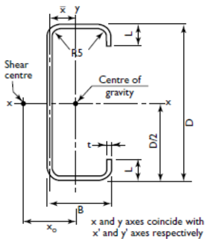
Cee section
