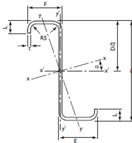
Zed section
